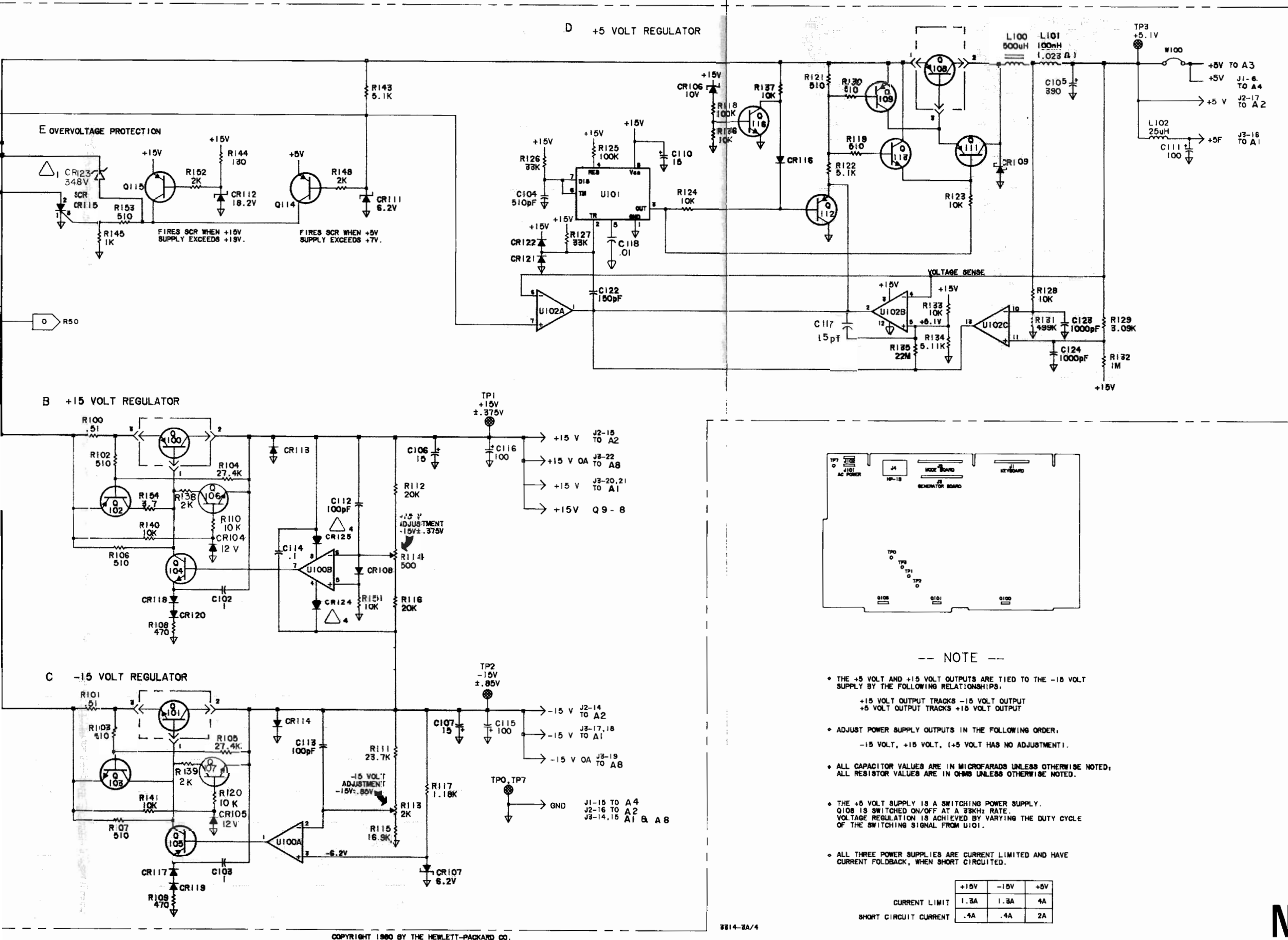
Figure 8-31. Power Supplies 8-69/8-70
